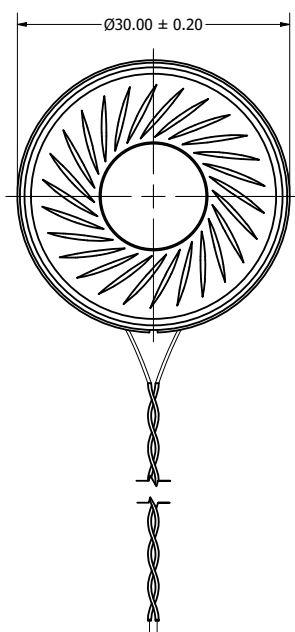
Top View
