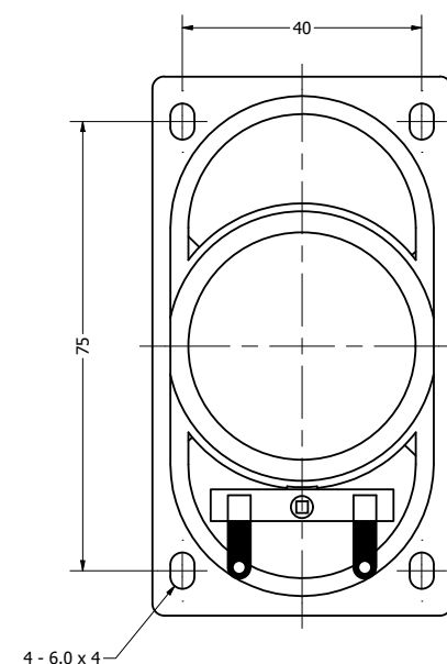
Bottom View
