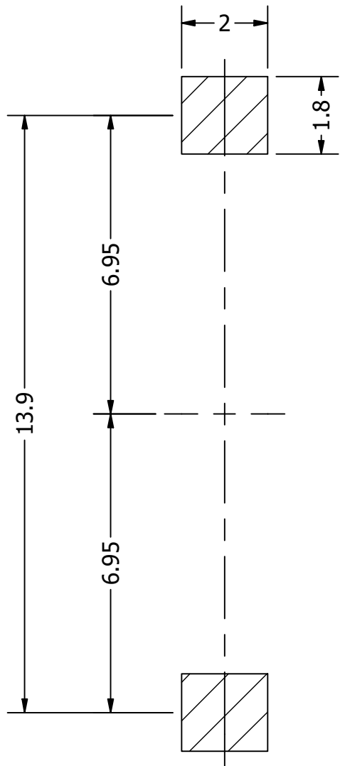
Suggested Pad Layout
